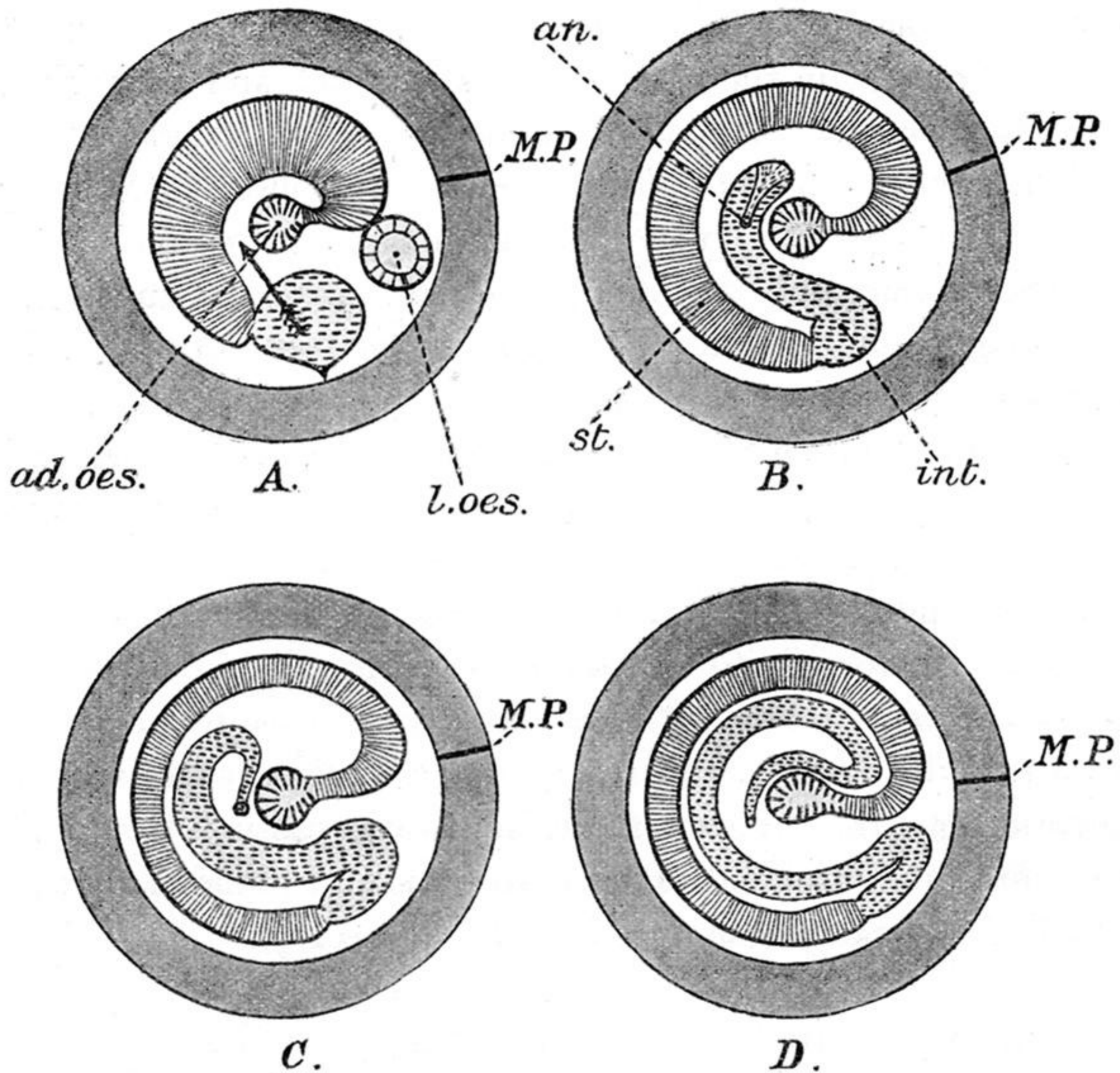
Fig. 6.—Four diagrams showing the manner in which the larval gut is transferred into the adult alimentary canal; ad. oes. , adult oesophagus; l. oes. , larval oesophagus; an. , annas; int. , intestine; st. , stomach; M.P., interradius in which the madreporite is situated. The arrow in diagram A shows the direction in which the anus migrates.
