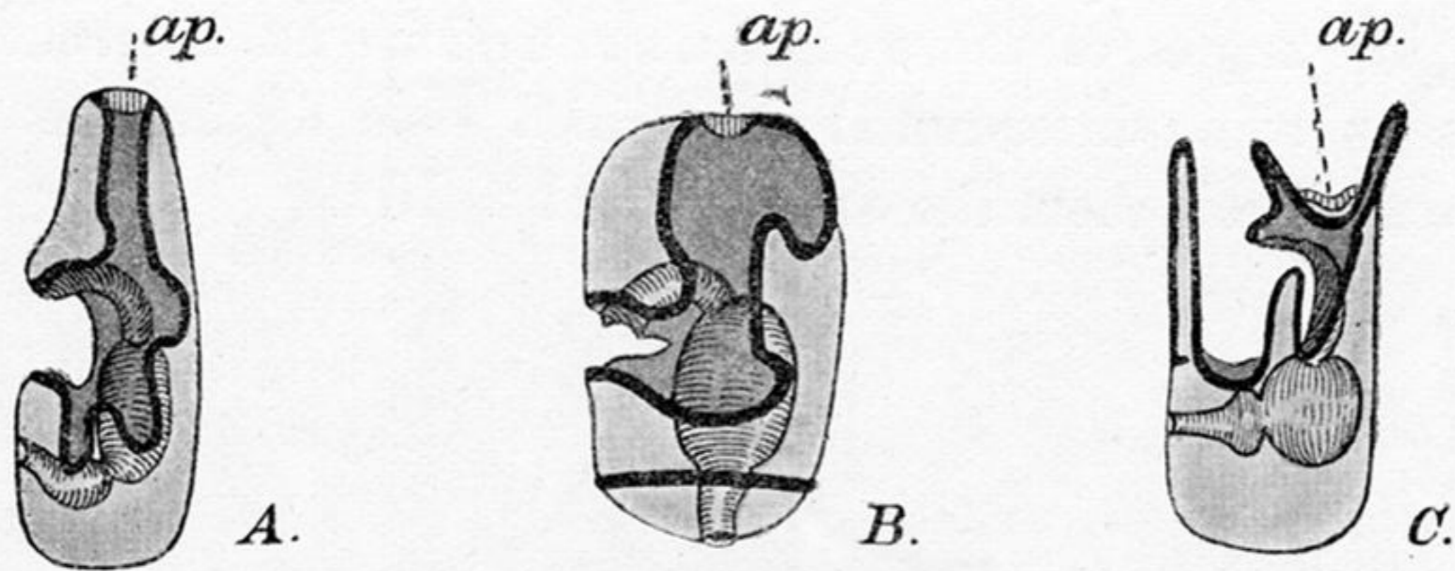
Fig. 3.—Three diagrams representing the side views of the Bipinnaria, the Tornaria, and the Echinopluteus larvæ respectively. A the Bipinnaria; B the Tornaria; C the Echinopluteus. The ciliated band is represented by a heavy line, and in the Echinopluteus the præ-oral loop of the ciliated band is very short. ap. , the apical nervous system.
