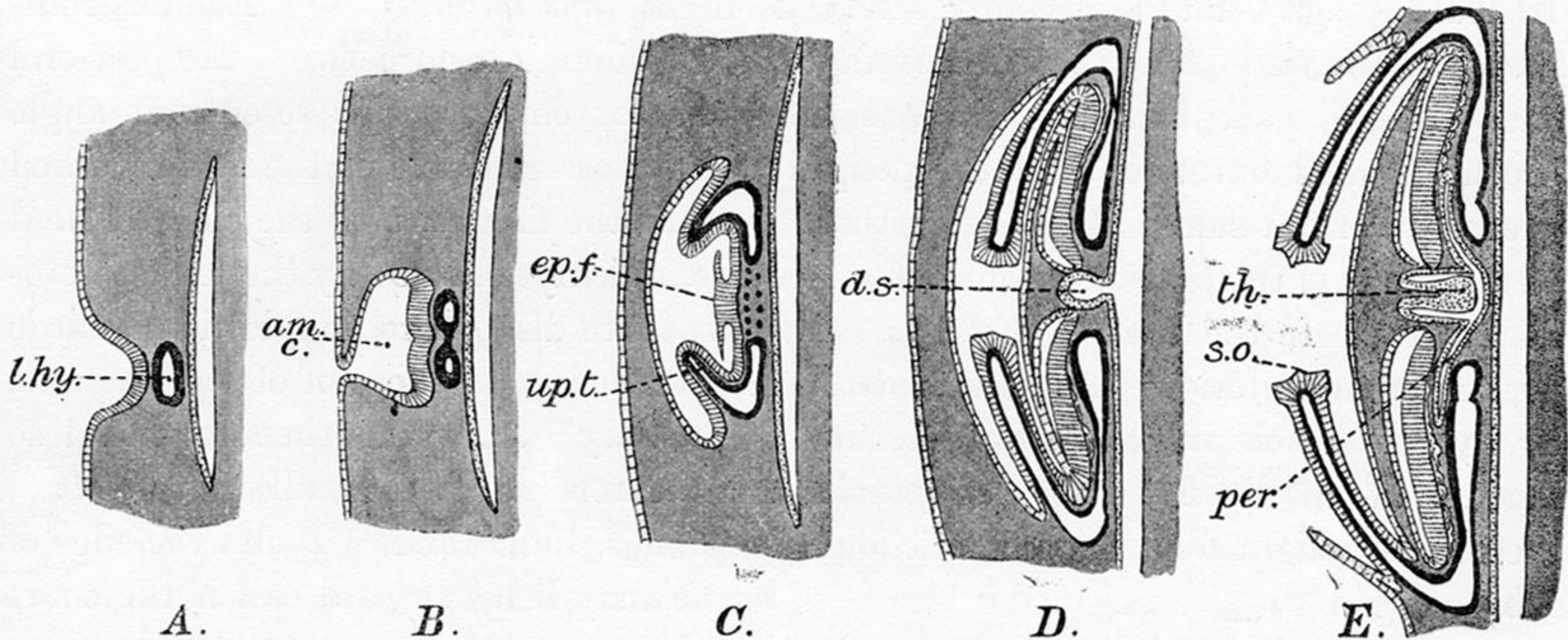
Fig. 5.—Five diagrams to show the gradual growth and differentiation of the echinus-rudiment. am. c. amniotic cavity; d. s. , dental sac; ep. f. , epineural fold; l. hy. , left hydrocoele; per. , rudiment of the perihæmal canal of the adult; s. o. , sense organ on apex of tube-foot; th. , rudiment of tooth; up. t. , unpaired tube-foot.
